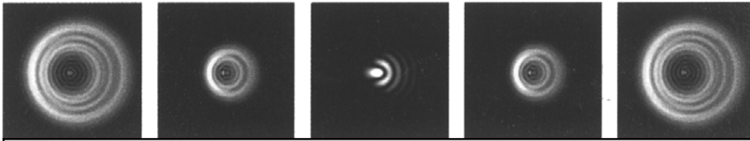
Fig 7-7 Even though the star pattern appears the same on both sides of focus, they are asymmetric. The dark obstruction is skewed off to the left side of the diffraction pattern indicating poor collimation.
